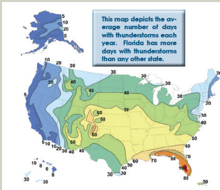
Figure 2-1. The average number of days with thunderstorms each year. Louisiana experiences between 60 and 70 thunderstorms annually. Preparing for larger hazard events can offer protection from these frequent storm events. Source: NOAA National Weather Service Southern Region Headquarters.
